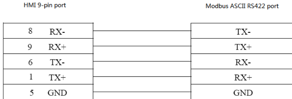
Fig2 Modbus RS422:
